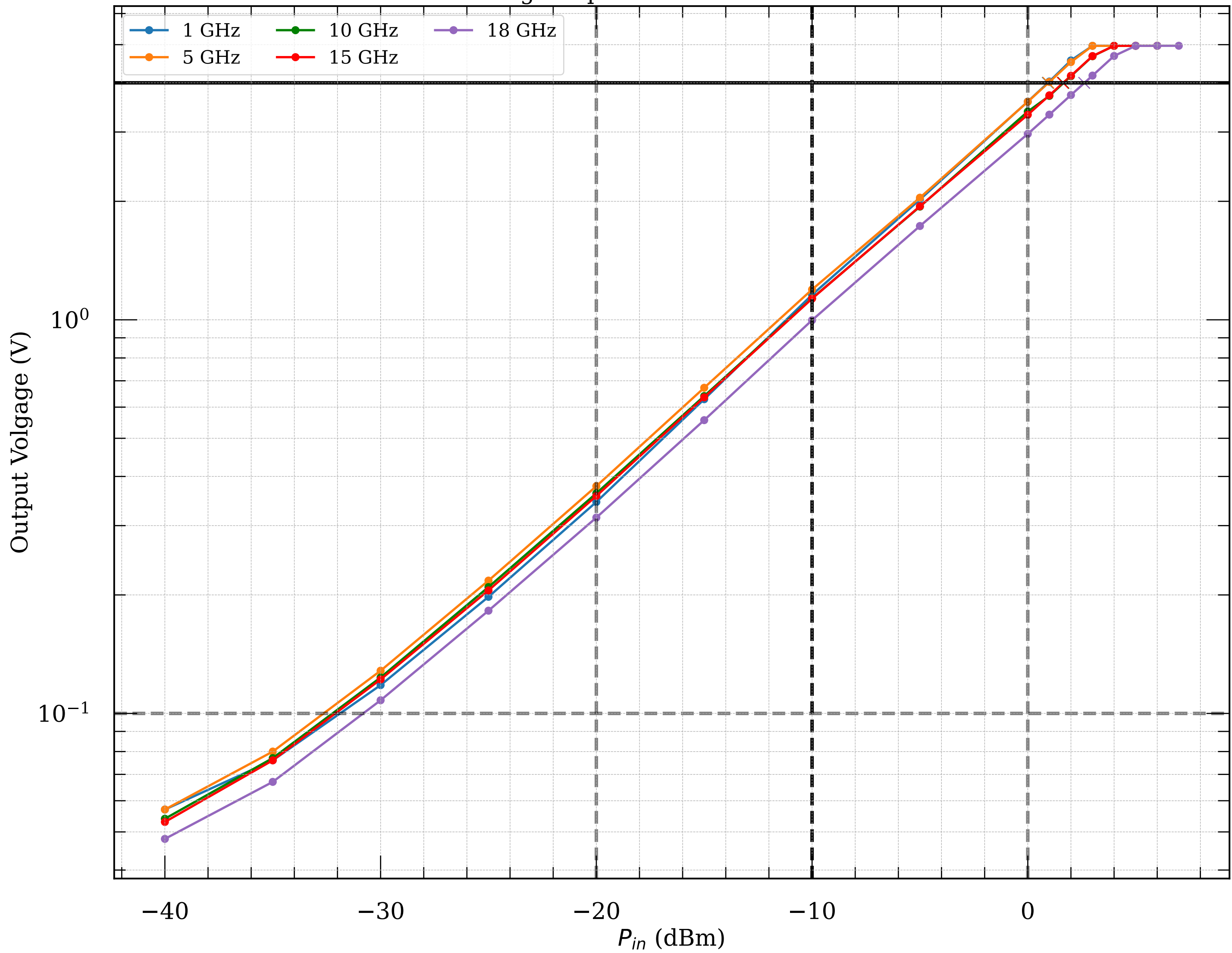
Measured voltage-to-power curve of detector module092
